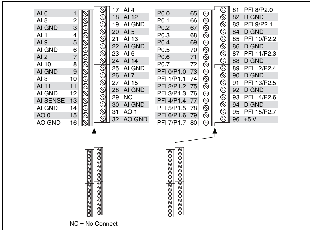
Figure A-4. USB-6221 Screw Terminal Pinout
