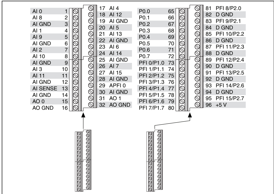
Figure A-29. USB-6251 Screw Terminal Pinout
