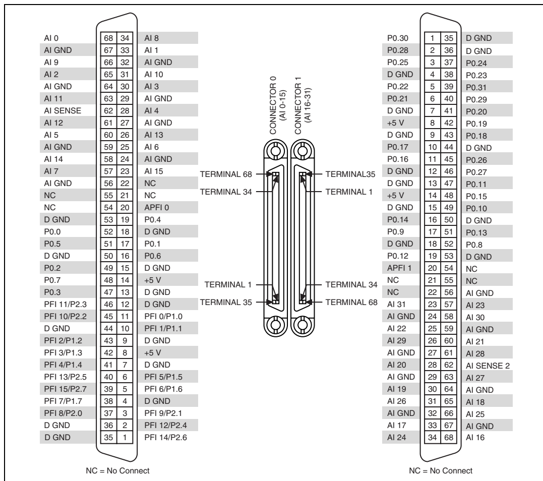
Figure A-58. PCI/PXI-6284 Pinout
