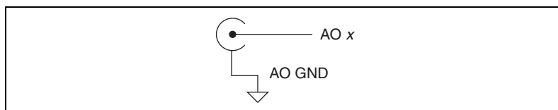
Figure A-23. Analog Output Circuitry
