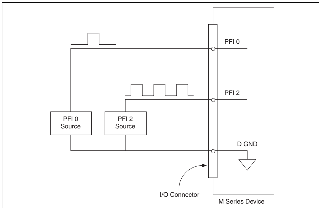
Figure 8-2. PFI Input Signals Connections
