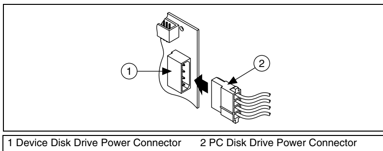
Figure 3-1. Connecting to the Disk Drive Power Connector
