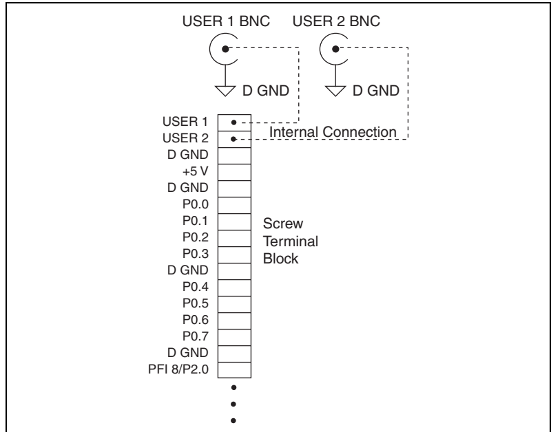
Figure A-37. USER <1..2> BNC Connections
