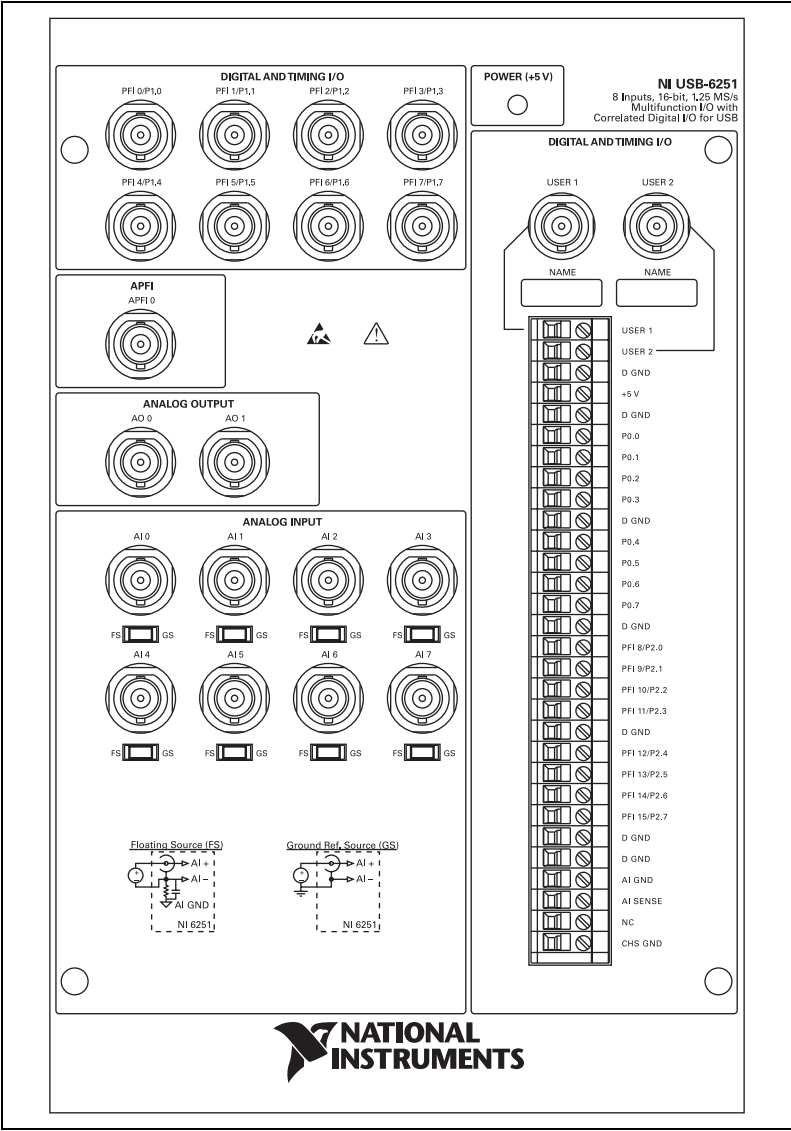
Figure A-30. USB-6251 BNC Top Panel and Pinout
