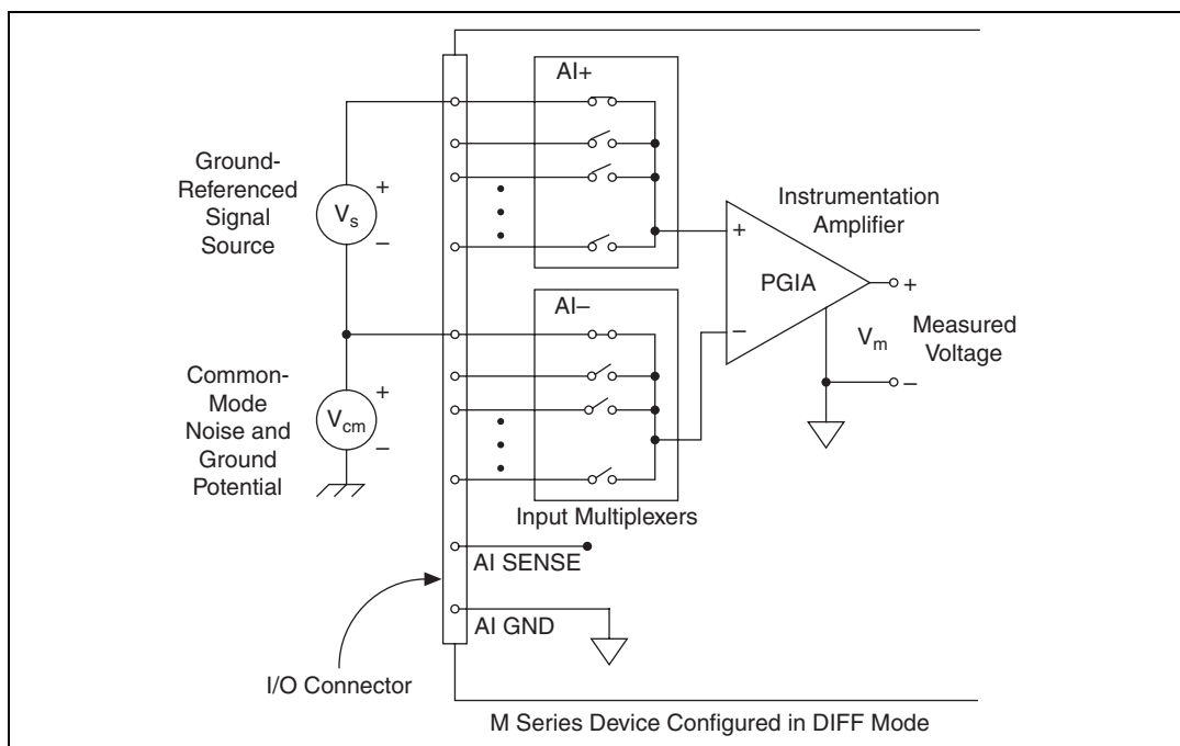
Figure 4-10. Differential Connections for Ground-Referenced Signal Sources
