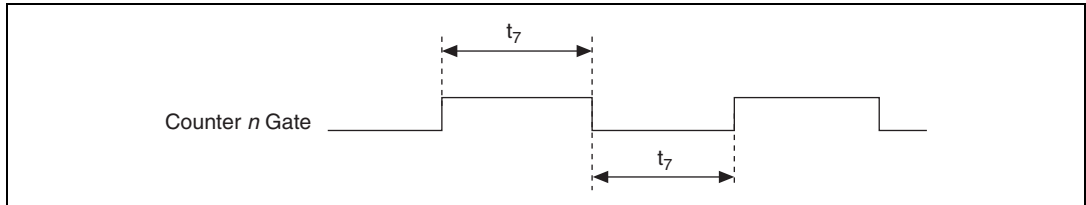
Figure B-47. Counter n Gate Pulse Width Timing Diagram
