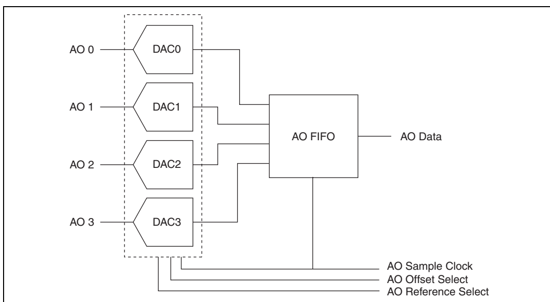
Figure 5-1. M Series Analog Output Circuitry
