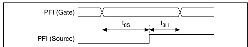
Figure B-48. Gate to Source Setup and Hold Timing Diagram
