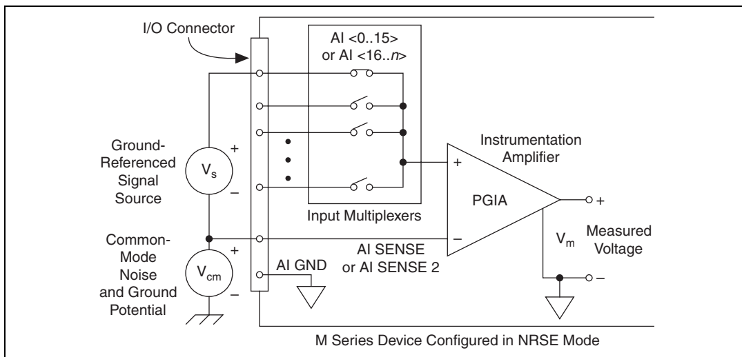
Figure 4-11. Single-Ended Connections for Ground-Referenced Signal Sources (NRSE Configuration)
