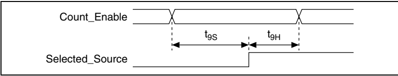
Figure B-49. DAQ-STC2 Internal Block Setup and Hold Requirements Timing Diagram
