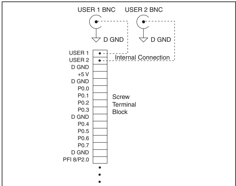
Figure A-25. USER <1..2> BNC Connections
