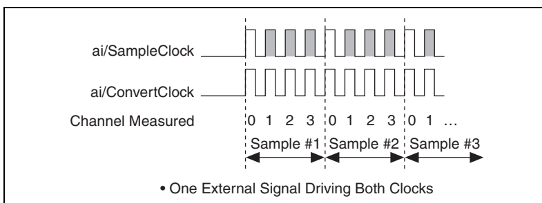
Figure 4-22. Single External Signal Driving ai/SampleClock and ai/ConvertClock Simultaneously
