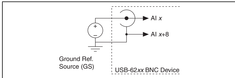
Figure A-49. Single-Ended Channels
