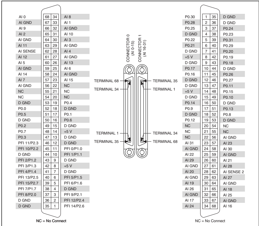
Figure A-13. PCI/PXI-6224 Pinout
