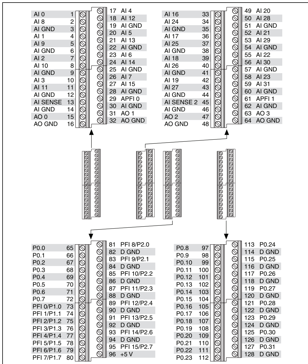
Figure A-45. USB-6259 Screw Terminal Pinout
