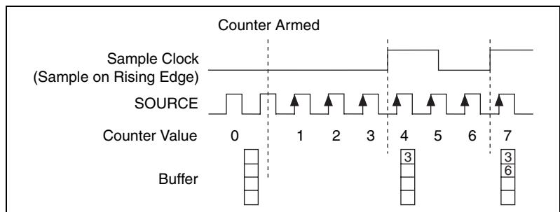
Figure 7-4. Buffered (Sample Clock) Edge Counting
