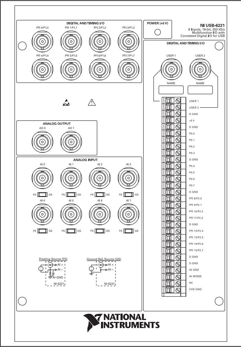
Figure A-5. USB-6221 BNC Top Panel and Pinout
