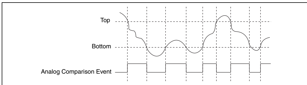
Figure 11-7. Analog Window Triggering Mode (Entering Window)
