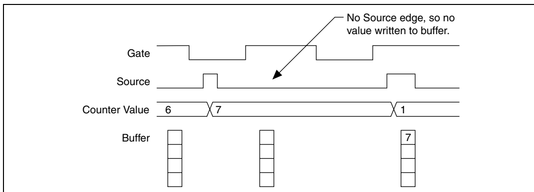
Figure 7-31. Duplicate Count Example
