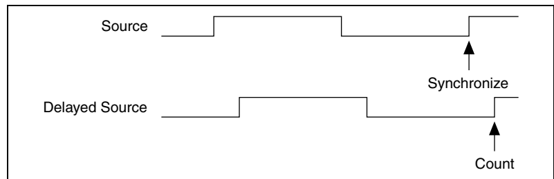
Figure 7-35. External Source Mode
