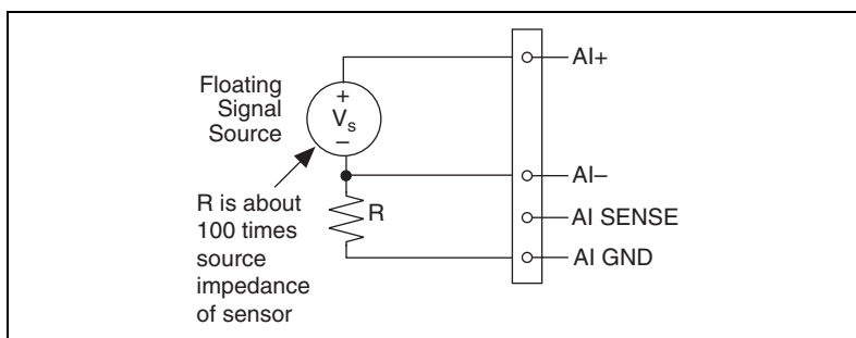
Figure 4-5. Differential Connections for Floating Signal Sources with Single Bias Resistor
