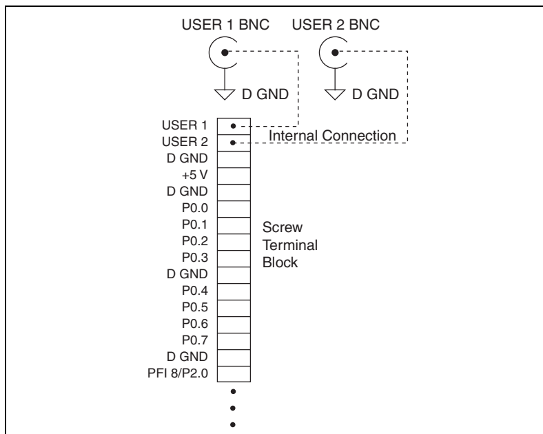
Figure A-53. USER <1..2> BNC Connections
