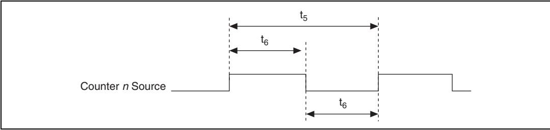
Figure B-46. Counter n Source Timing Requirements
