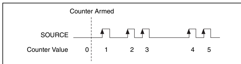
Figure 7-2. Single Point (On-Demand) Edge Counting
