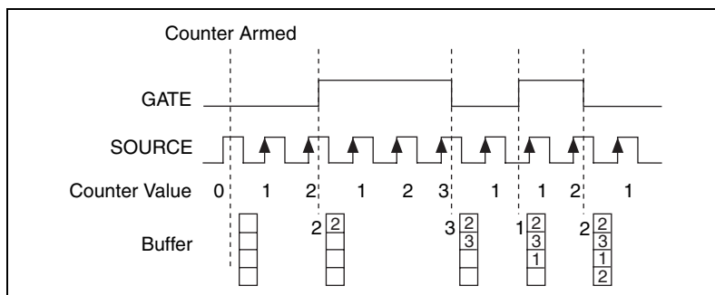
Figure 7-9. Buffered Semi-Period Measurement
