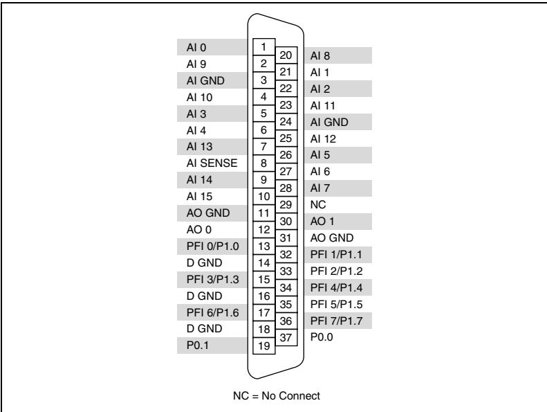
Figure A-3. PCI-6221 (37-Pin) Pinout
