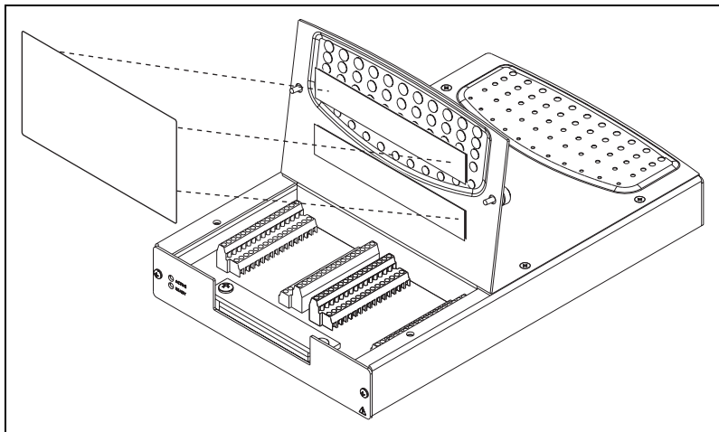
Figure 1-1. Applying the USB-622x/625x Screw Terminal Signal Label
