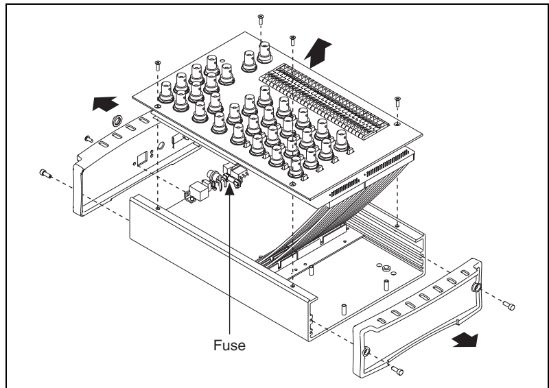
Figure 3-3. USB-62xx BNC Fuse Location
