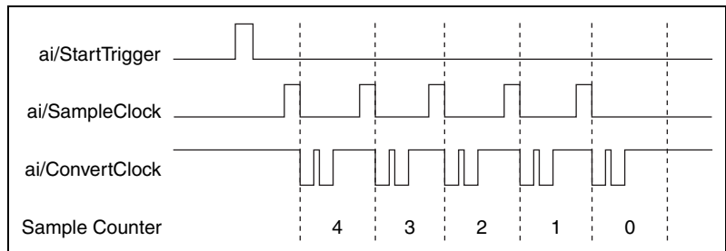
Figure 4-14. Posttriggered Data Acquisition Example
