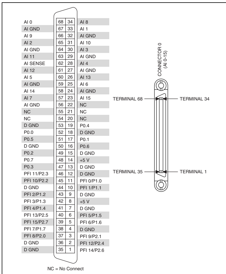
Figure A-1. PCI/PXI-6220 Pinout
