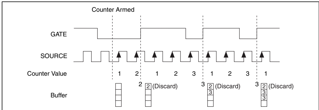
Figure 7-8. Buffered Period Measurement
