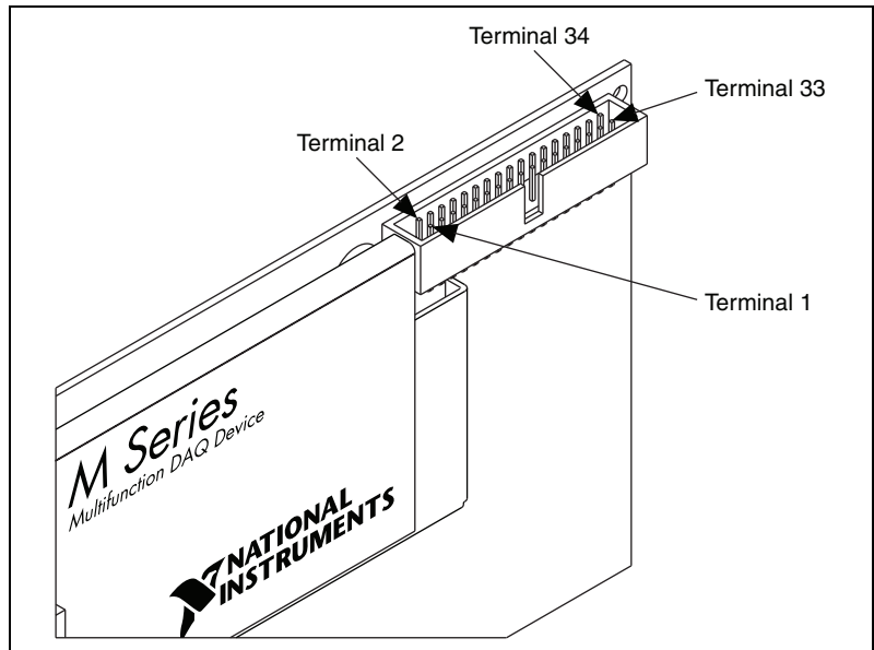
Figure 9-2. M Series RTSI Pinout
