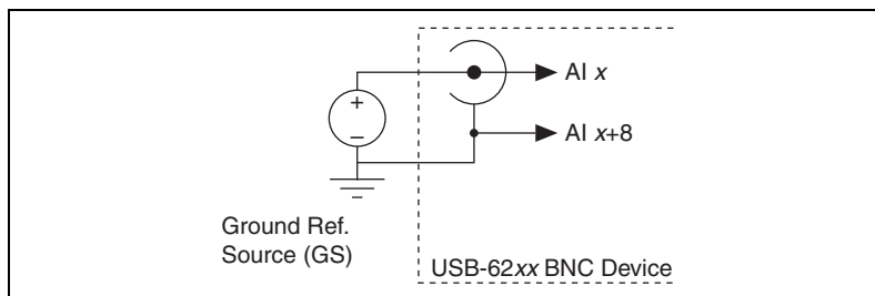
Figure A-22. Single-Ended Channels
