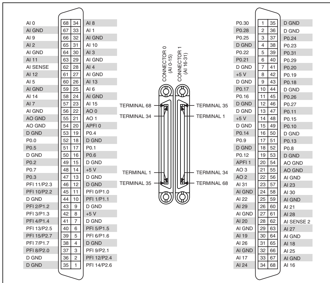
Figure A-59. PCI/PXI-6289 Pinout
