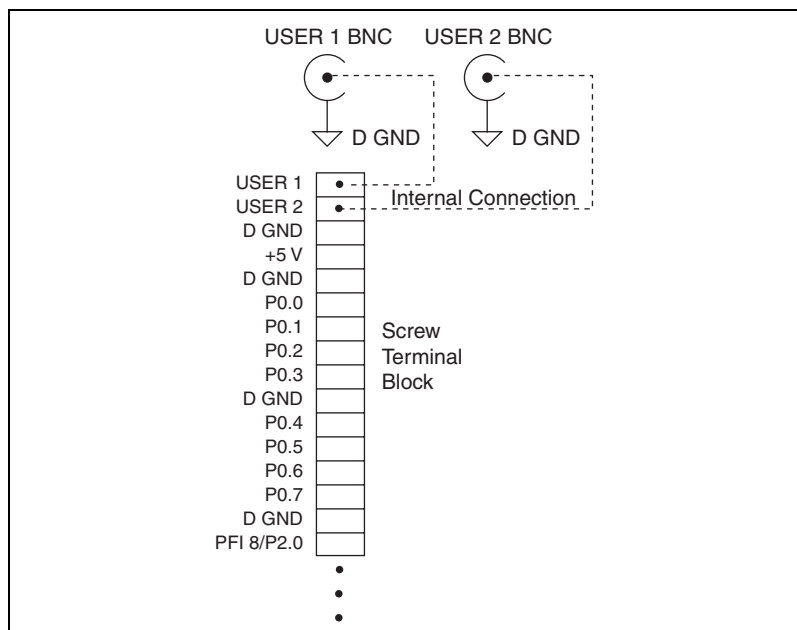
Figure A-11. USER <1..2> BNC Connections
