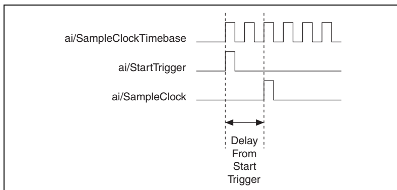
Figure 4-16. ai/SampleClock and ai/StartTrigger
